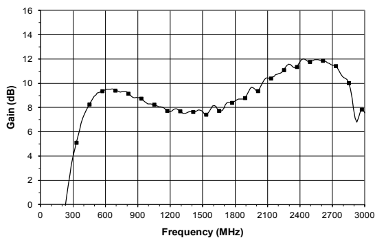
Figure 30: Gain vs. Frequency
